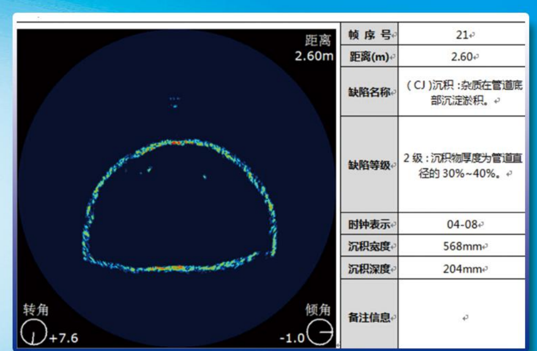
Pipe deformation and branch secret joint
